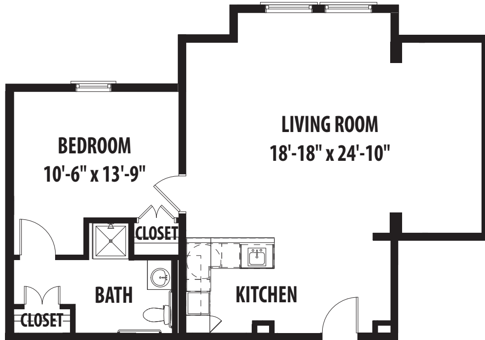
1/8" SCALE - DIMENSIONS SUBJECT TO CHANGE SQUARE FOOTAGE IS APPROXIMATE
